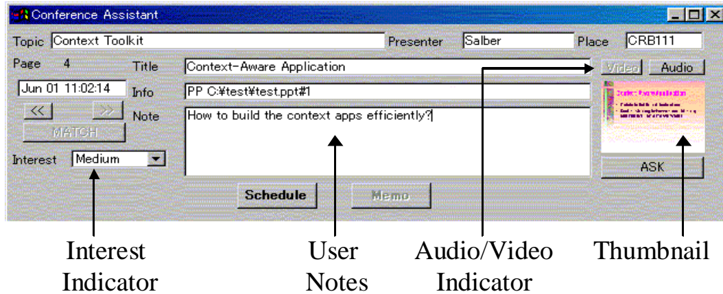
Figure 13. Screenshot of the Conference Assistant note taking interface.
