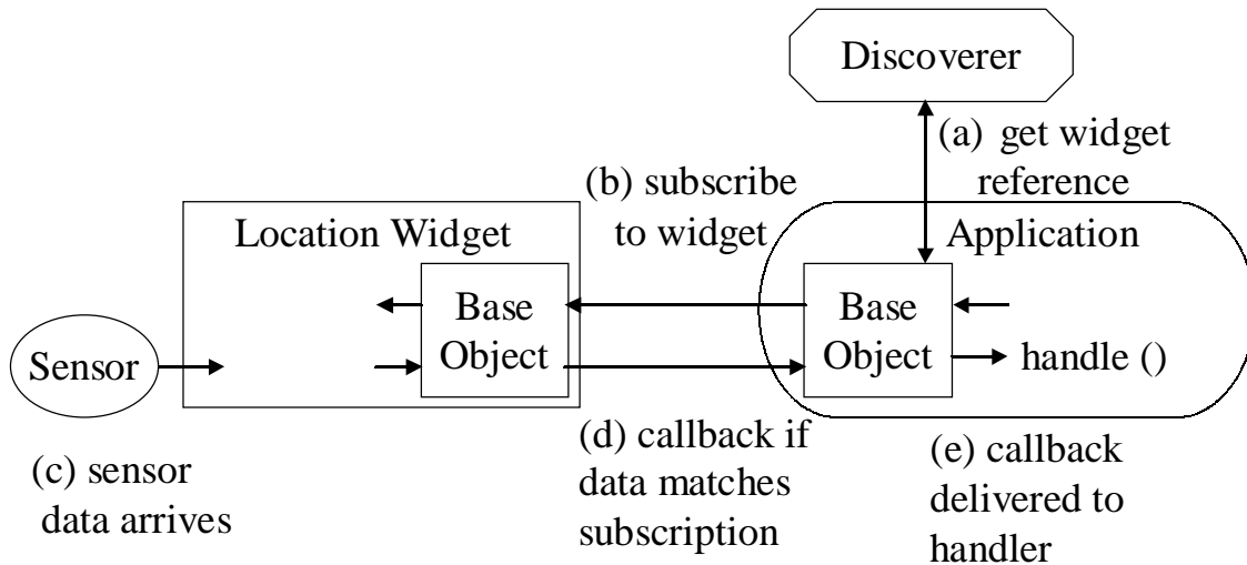
Figure 5. Application subscribing to a context widget.
