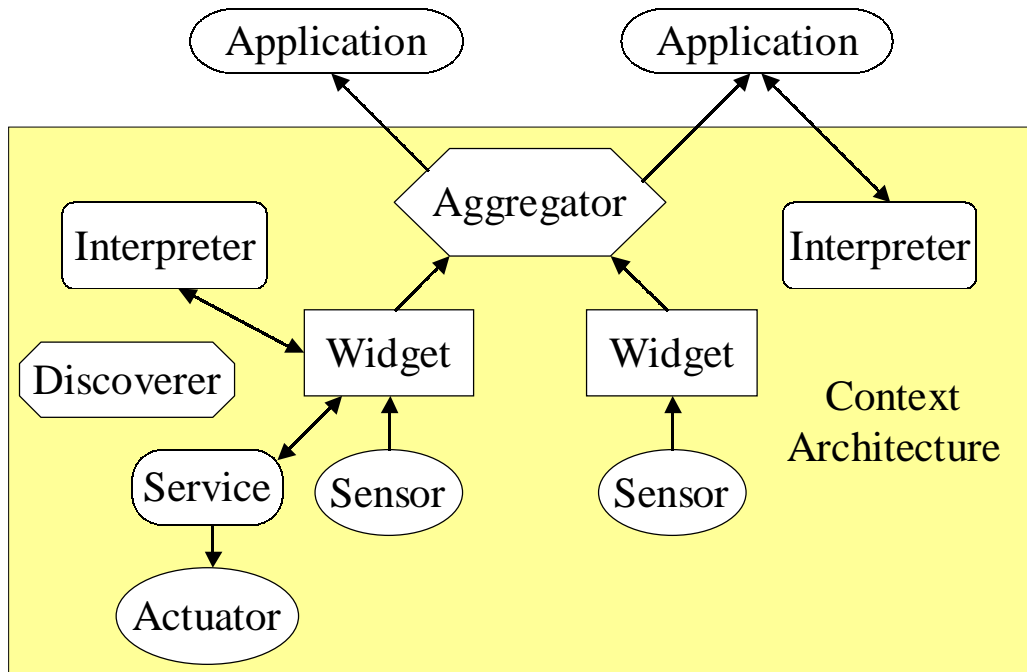
Figure 1. Example configuration of Context Toolkit components
