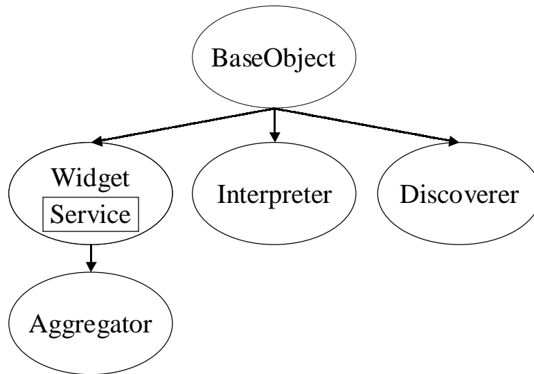
Figure 4. Object diagram for the Context Toolkit abstractions.
