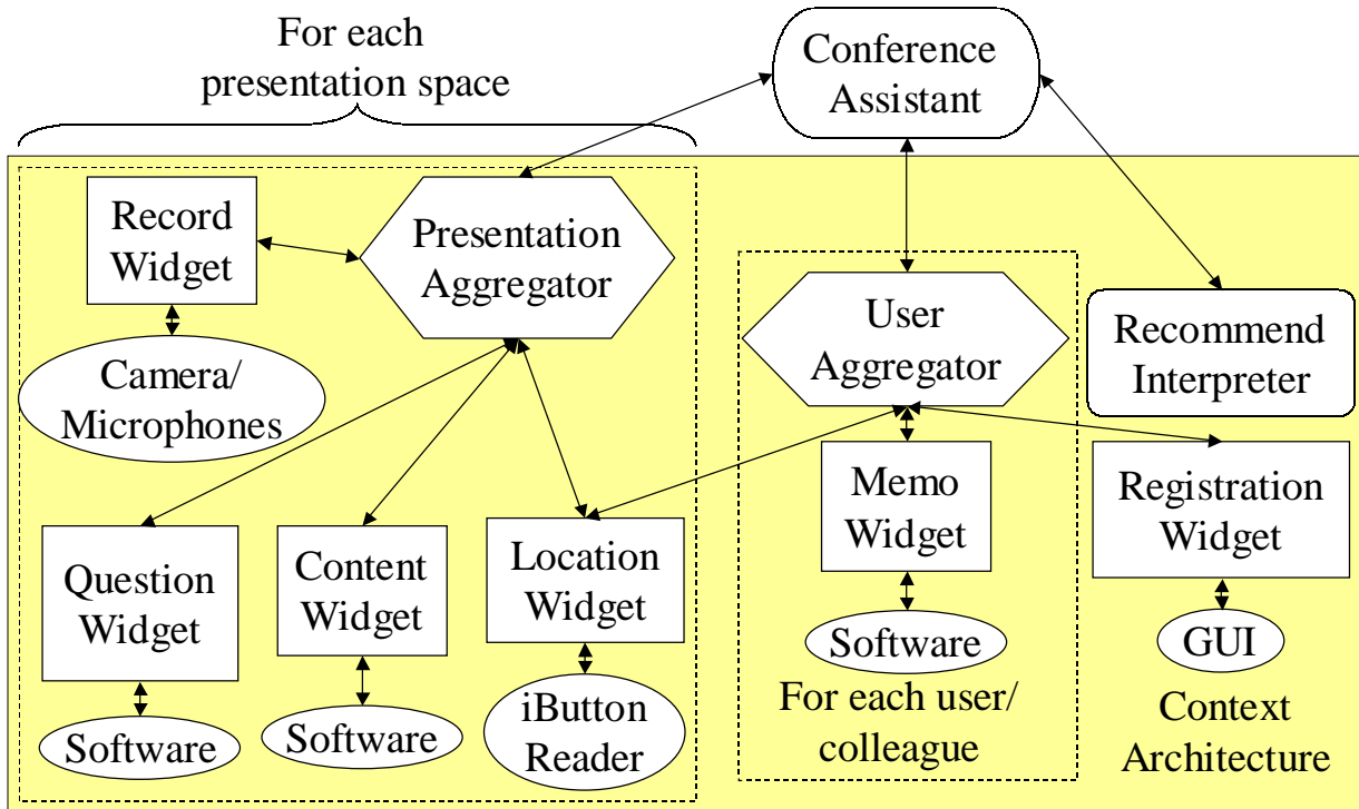
Figure 19. Conference Assistant context architecture.
