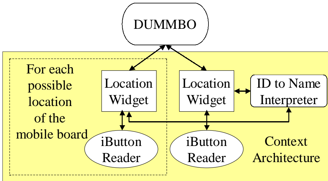
Figure 10. Context architecture for the DUMMBO application.
