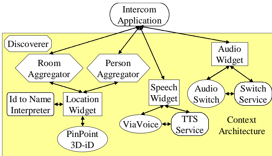
Figure 11. Architecture diagram for the Intercom application.
